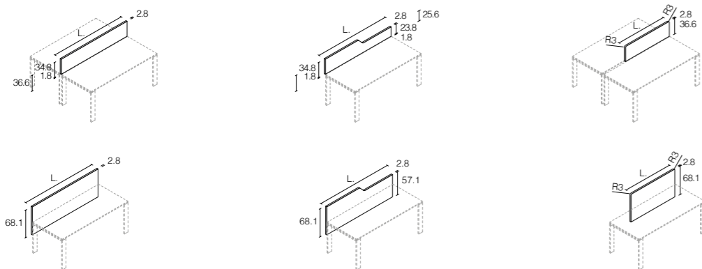
Screen sospesi in melaminico Melamine not floor-level screens
