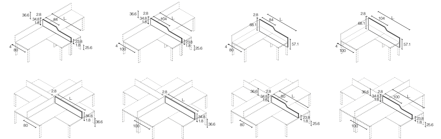
Screen laterale in melaminico per scrivanie dotate di dattilo e screen lato lungo Melamine side screen for desk with type-desk and screen on the longer side
