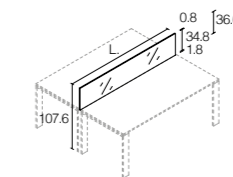
Screen sospesi in vetro Glass not floor-level screens
