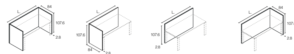
Screen a pavimento in melaminico per reception Melamine floor-level screens for reception
